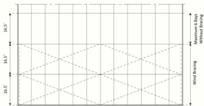
98' Structure Top Elevation
