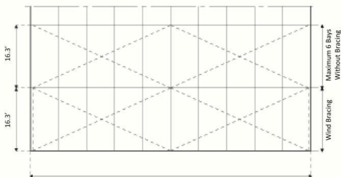
82' Structure Top Elevation
