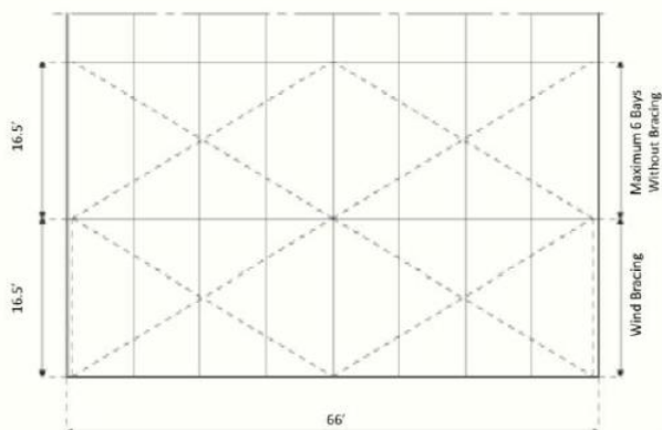
66' Structure Top Elevation
