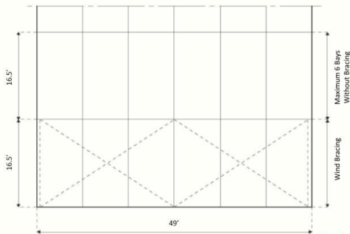
49' Structure Top Elevation
