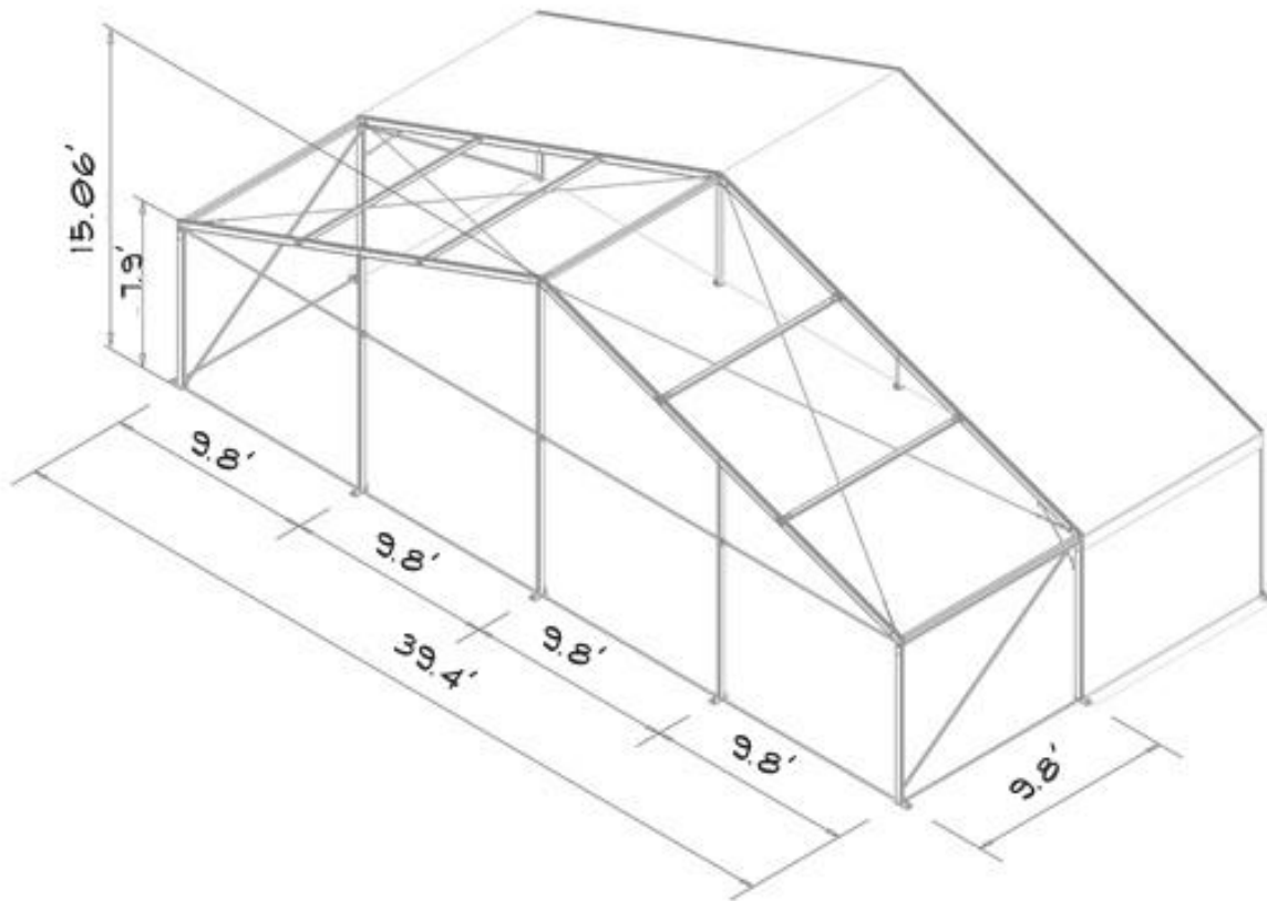
Framing Plan
